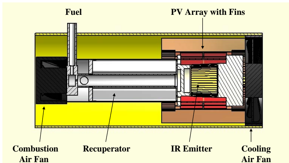
Cross section of TPV generator cylinder.
